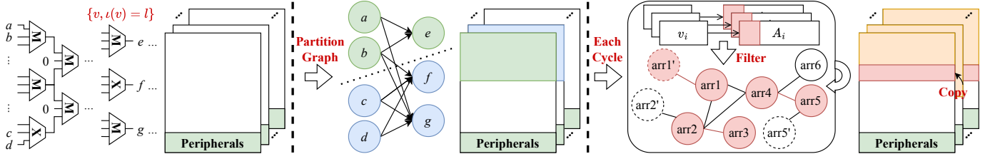
Fig. 3. MAPSIM overall flow.
