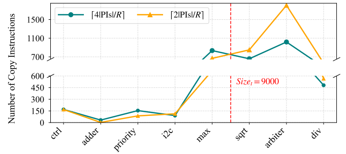
Fig. 11. Number of copy instructions of the two k -value selection methods, with EPFL [30] circuits arranged in ascending order of vertex count.
