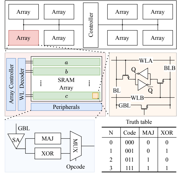
Fig. 2. IMC hardware architecture. (SA: sense amplifier, N: number of ‘1’s, Code: thermometer code of SA output voltage).
