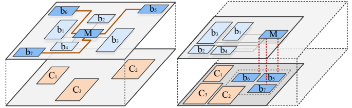
Fig. 1 Comparison of 3D floorplans before and after inter-die optimization. Our method (right) better utilizes vertical links and achieves reduced area under identical outline constraints.
