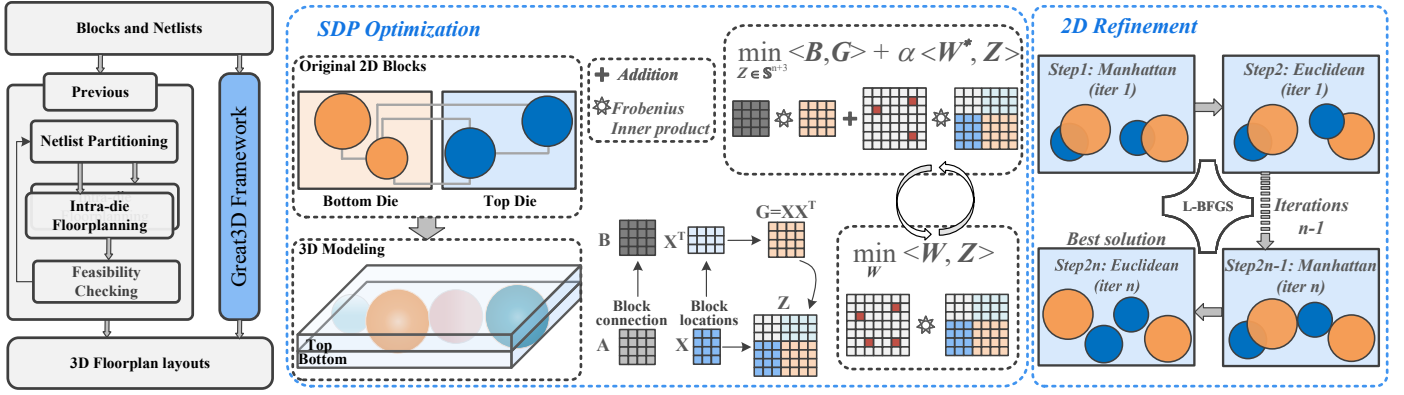
Fig. 2 Overview of the proposed GREAT3D optimization framework shown in Section III. The framework consists of two key components: SDP-based optimization (Section III-A) and 2D refinement (Section III-B).
